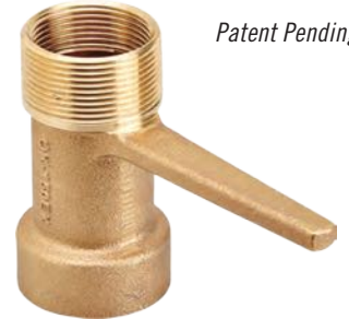
1 1/2" MPT x 1 1/4" FPT outlet 1 1/2" FPT inlet Part # QK-150EX
